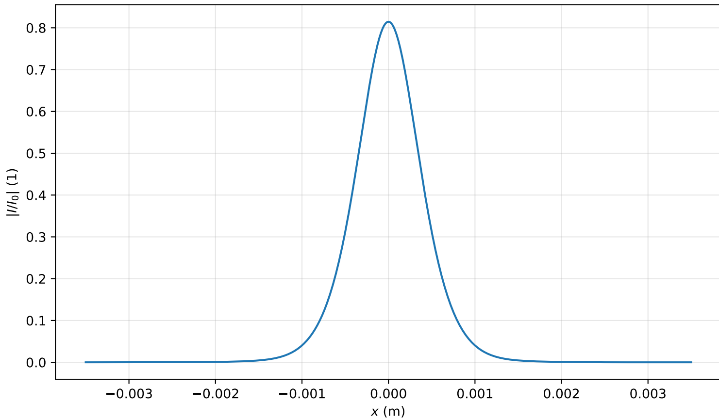
Intensity profile I(x, y = 0, z = 3.105m)/I_0 , P_{in}=0.7P_{cr} , artificial time
